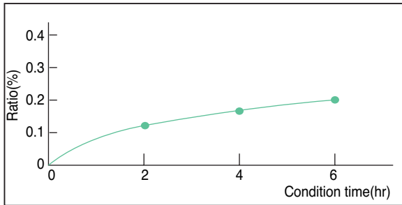
■ Water absorption(D-X/100)
